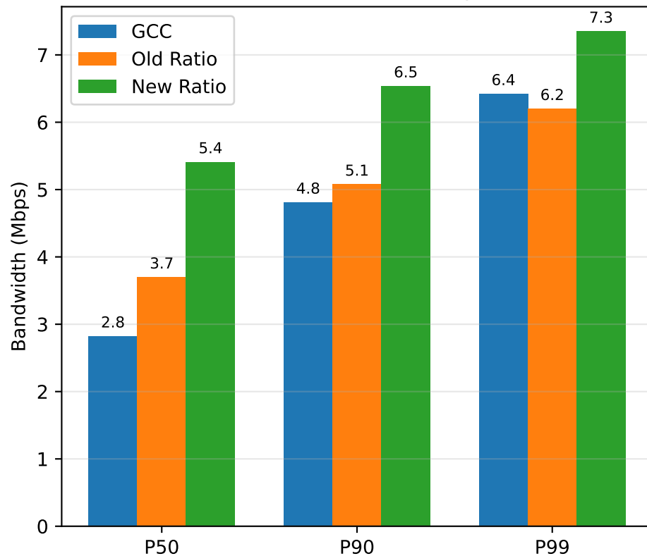
Bandwidth Percentile Comparison
